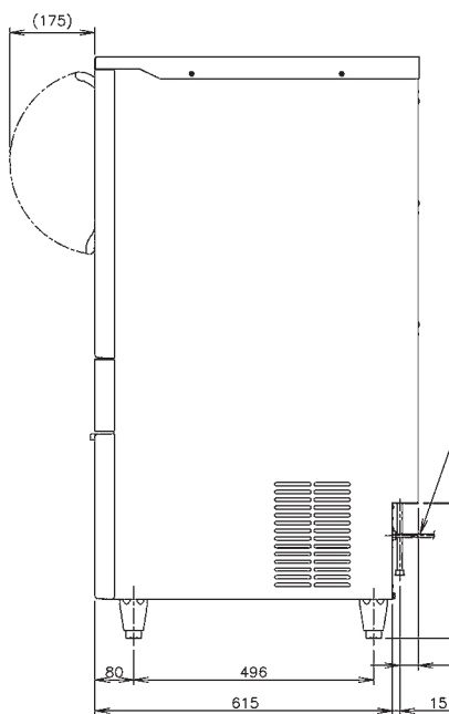
RIGHT SIDE
